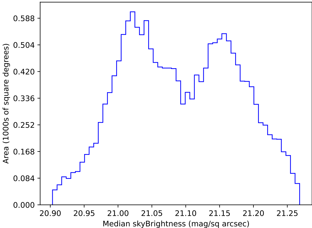
too_elab_r128_d2_gz_v3.4_10yrs WFD r band: Median skyBrightness
