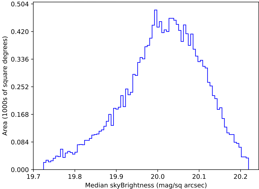
too_elab_r128_d2_gz_v3.4_10yrs WFD i band: Median skyBrightness
