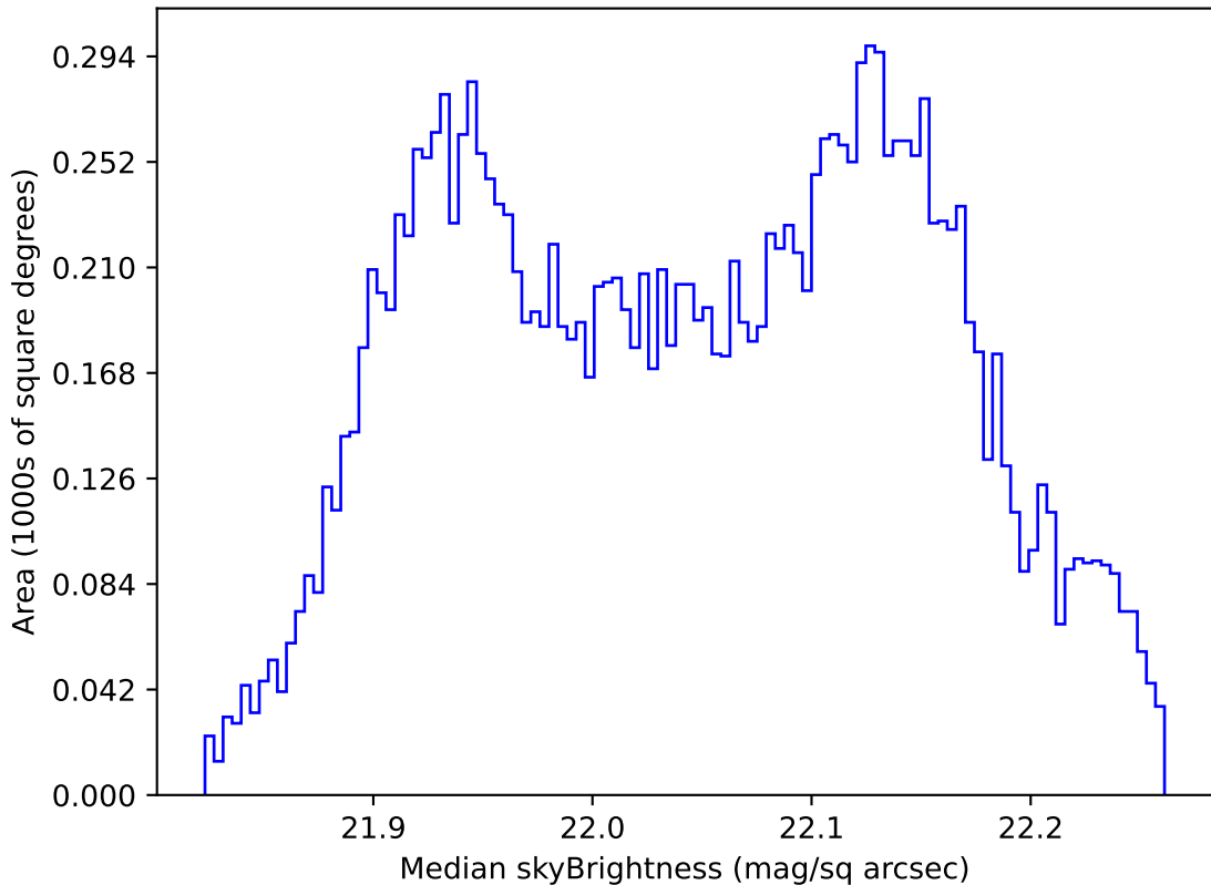
too_elab_r128_d2_gz_v3.4_10yrs WFD g band: Median skyBrightness
