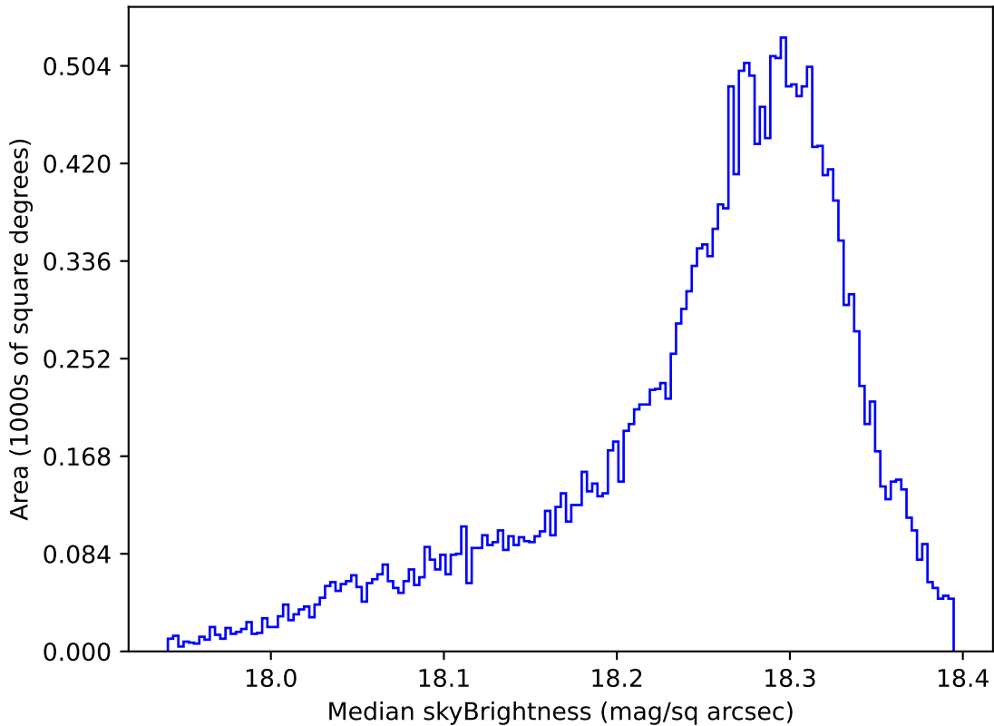
too_elab_r128_d2_gz_v3.4_10yrs All sky y band: Median skyBrightness
