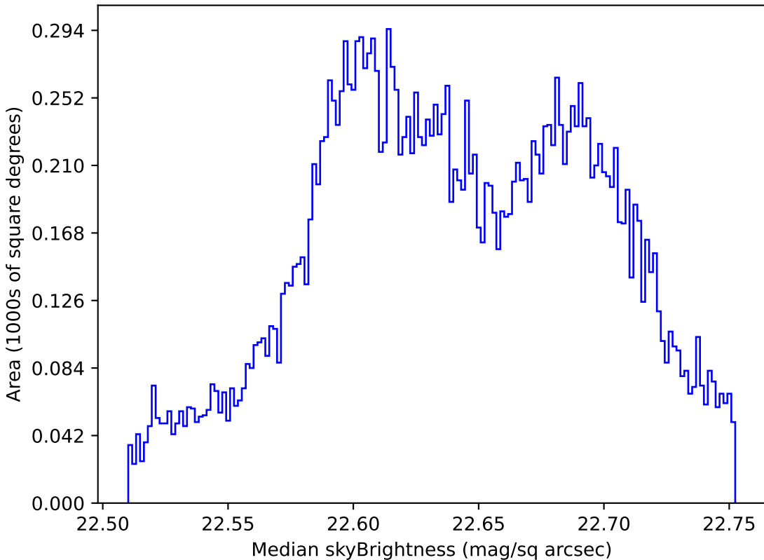
too_elab_r128_d2_gz_v3.4_10yrs All sky u band: Median skyBrightness
