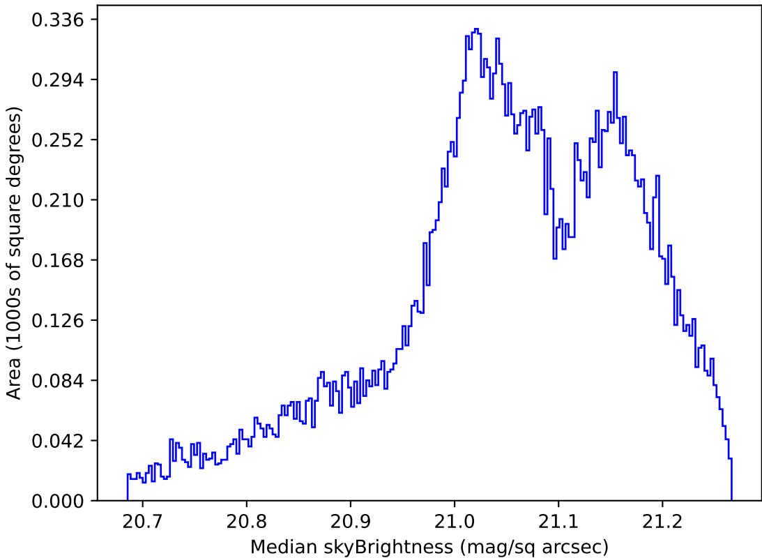
too_elab_r128_d2_gz_v3.4_10yrs All sky r band: Median skyBrightness
