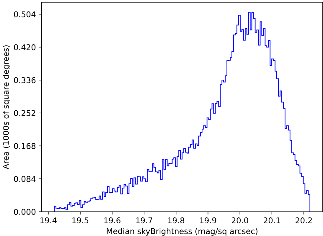
too_elab_r128_d2_gz_v3.4_10yrs All sky i band: Median skyBrightness
