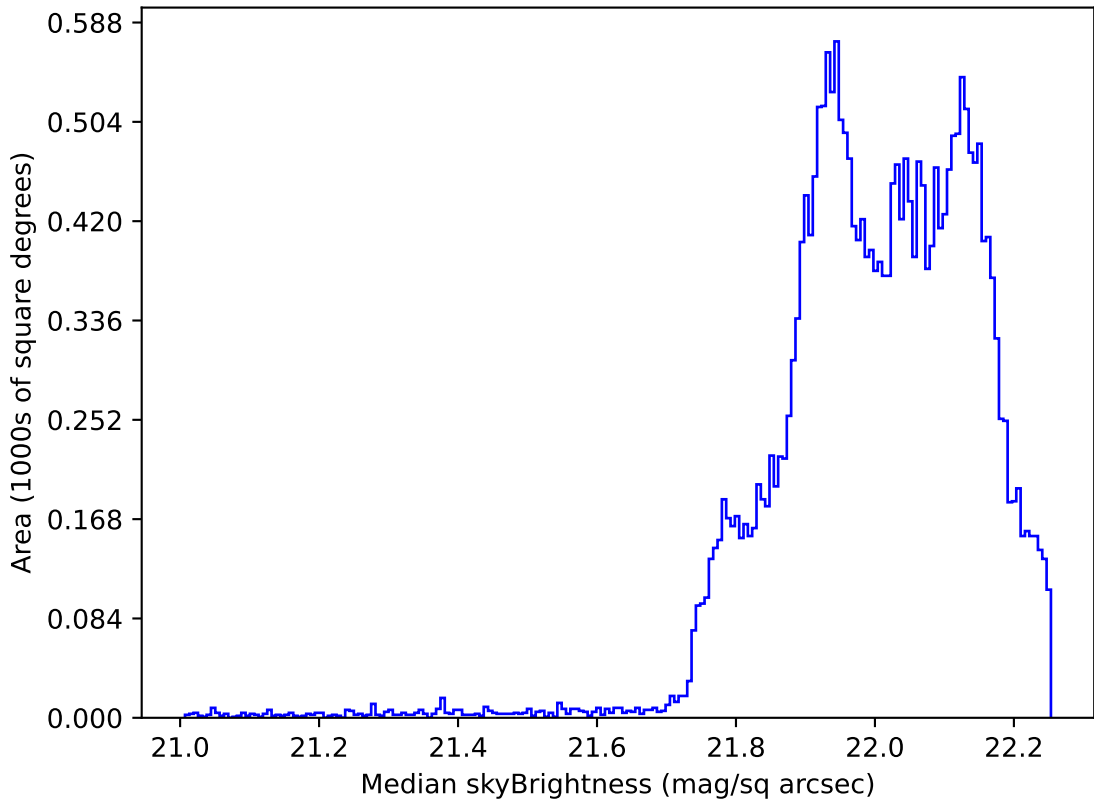
too_elab_r128_d2_gz_v3.4_10yrs All sky g band: Median skyBrightness
