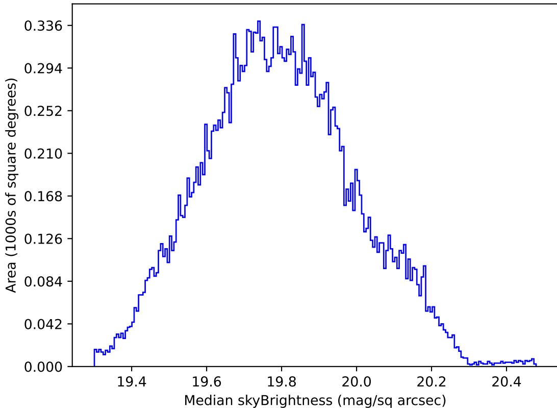
too_elab_r128_d2_gz_v3.4_10yrs All sky all bands: Median skyBrightness
