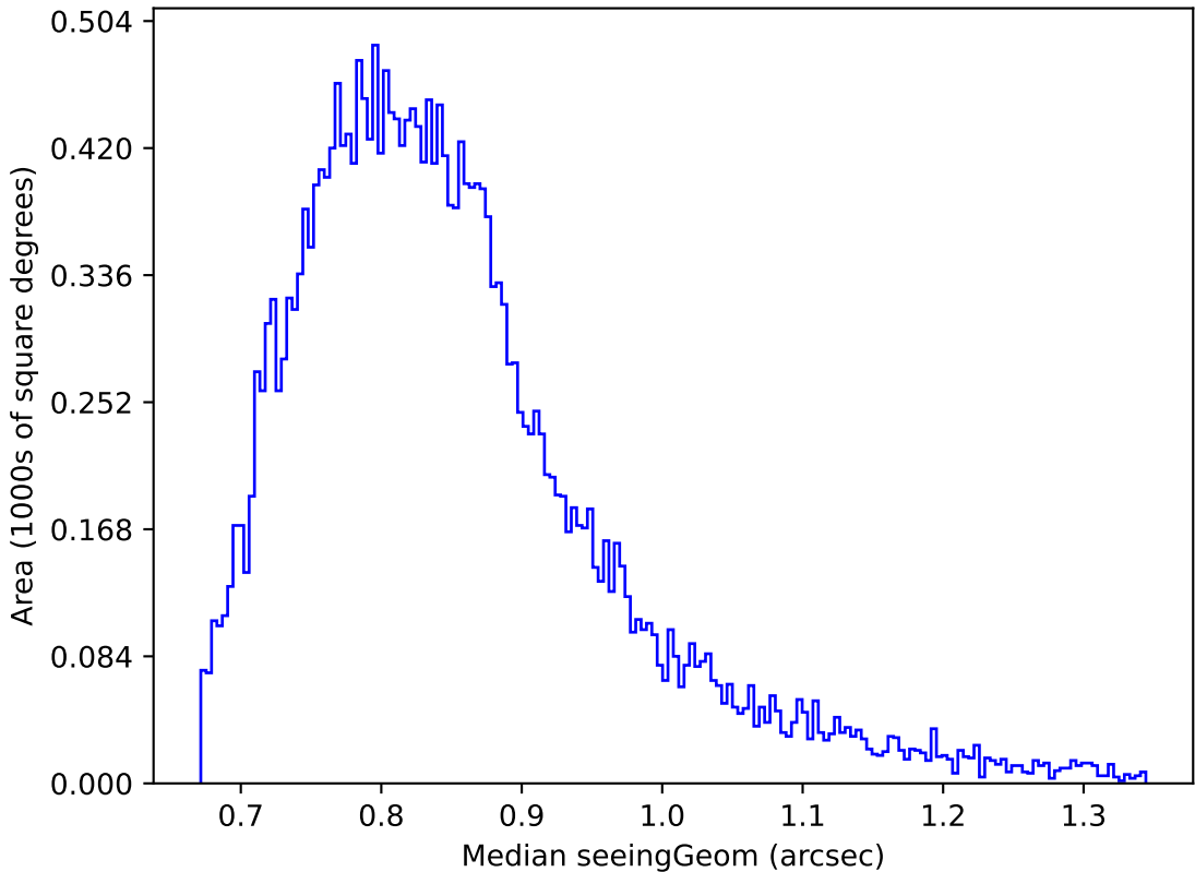
too_elab_r128_d2_gz_v3.4_10yrs Yr 1 z band: Median seeingGeom
