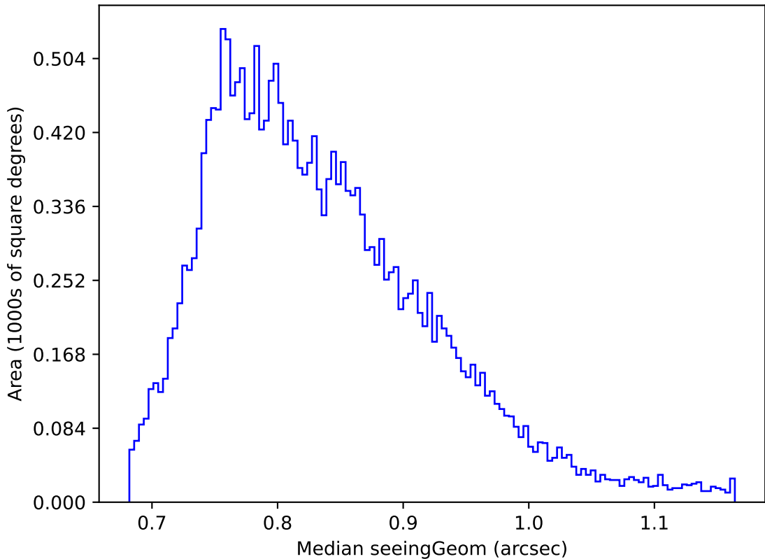
too_elab_r128_d2_gz_v3.4_10yrs Yr 1 y band: Median seeingGeom
