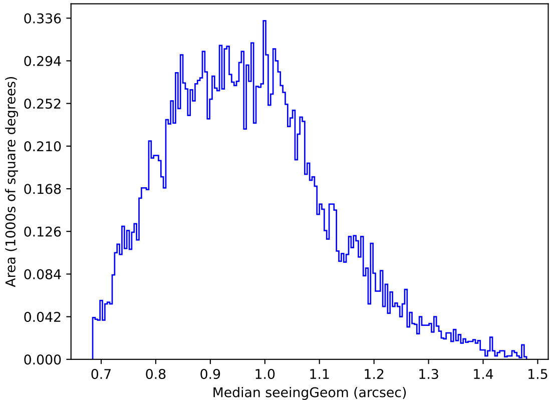
too_elab_r128_d2_gz_v3.4_10yrs Yr 1 u band: Median seeingGeom
