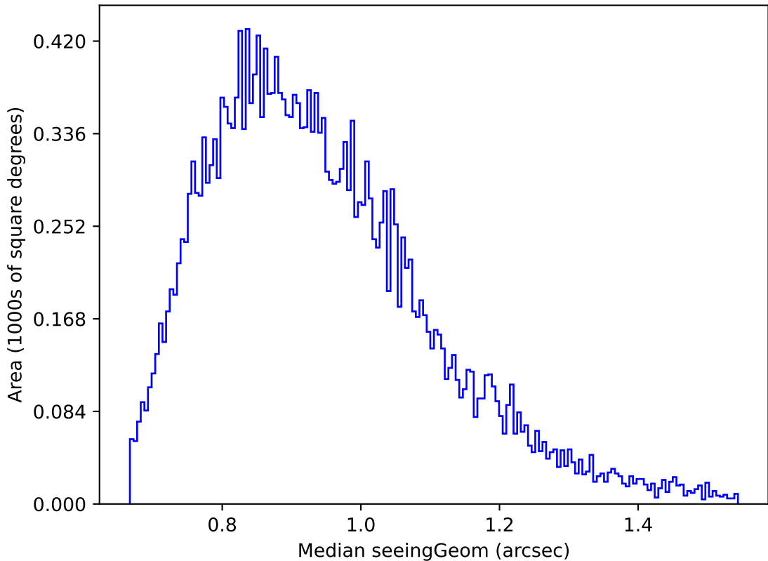
too_elab_r128_d2_gz_v3.4_10yrs Yr 1 g band: Median seeingGeom
