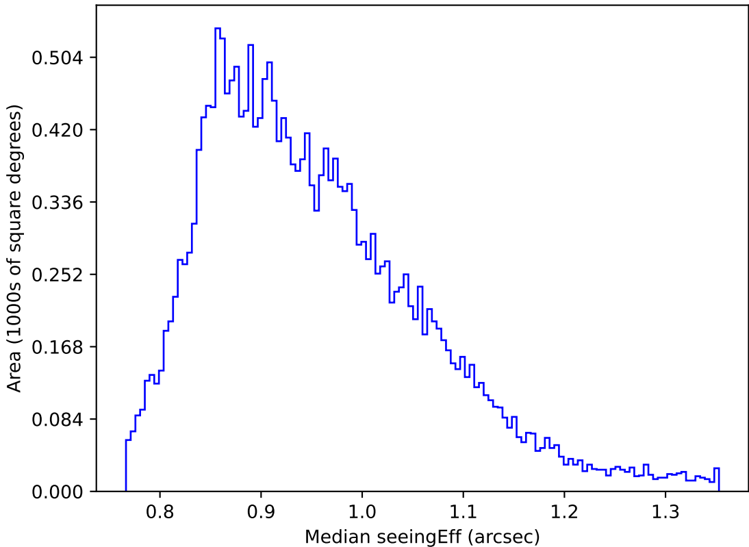
too_elab_r128_d2_gz_v3.4_10yrs Yr 1 y band: Median seeingEff
