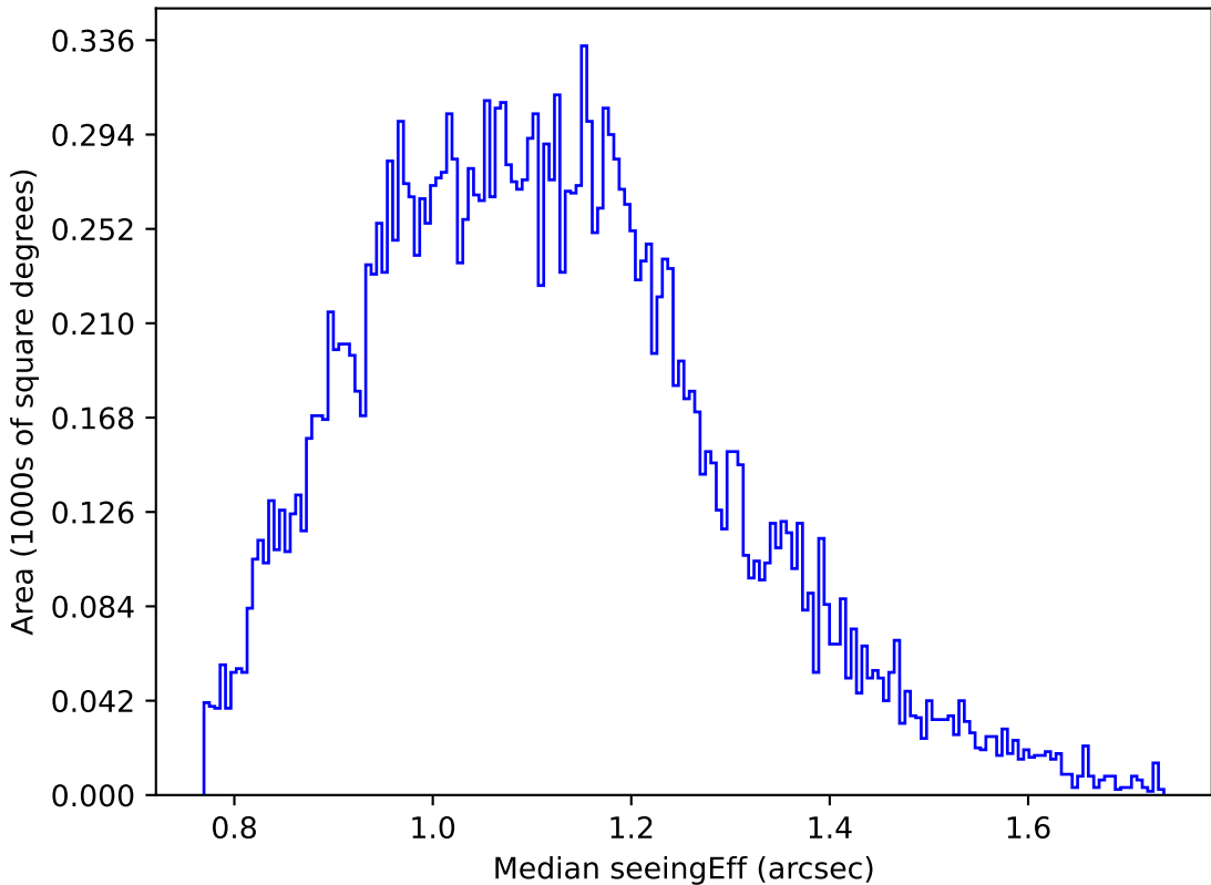
too_elab_r128_d2_gz_v3.4_10yrs Yr 1 u band: Median seeingEff
