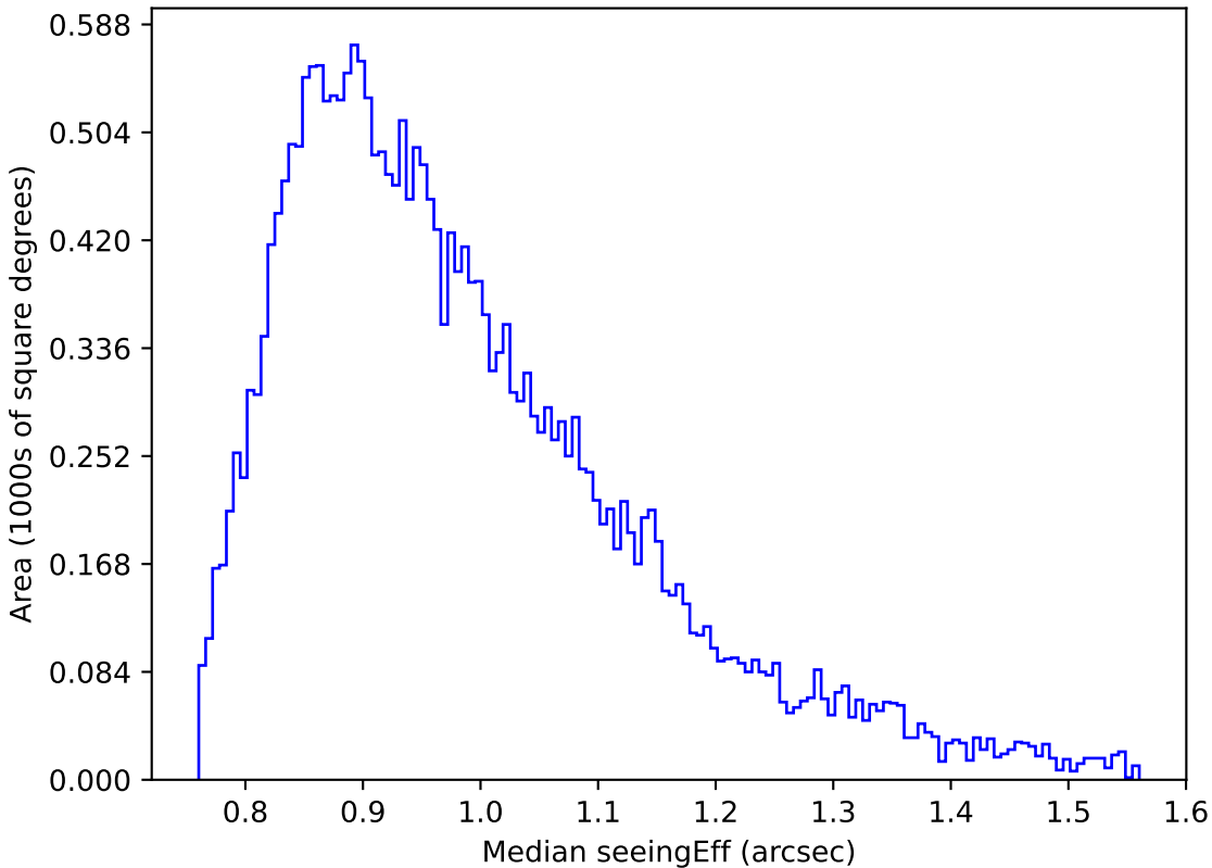
too_elab_r128_d2_gz_v3.4_10yrs Yr 1 r band: Median seeingEff
