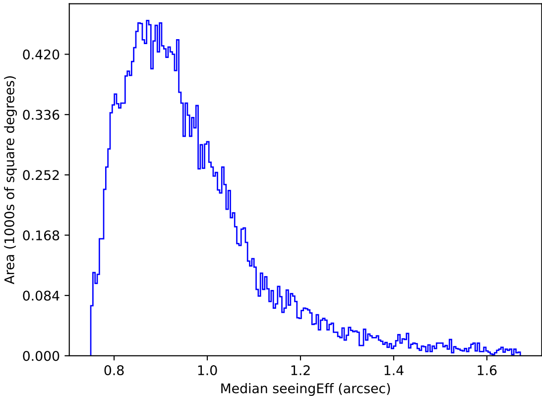
too_elab_r128_d2_gz_v3.4_10yrs Yr 1 i band: Median seeingEff
