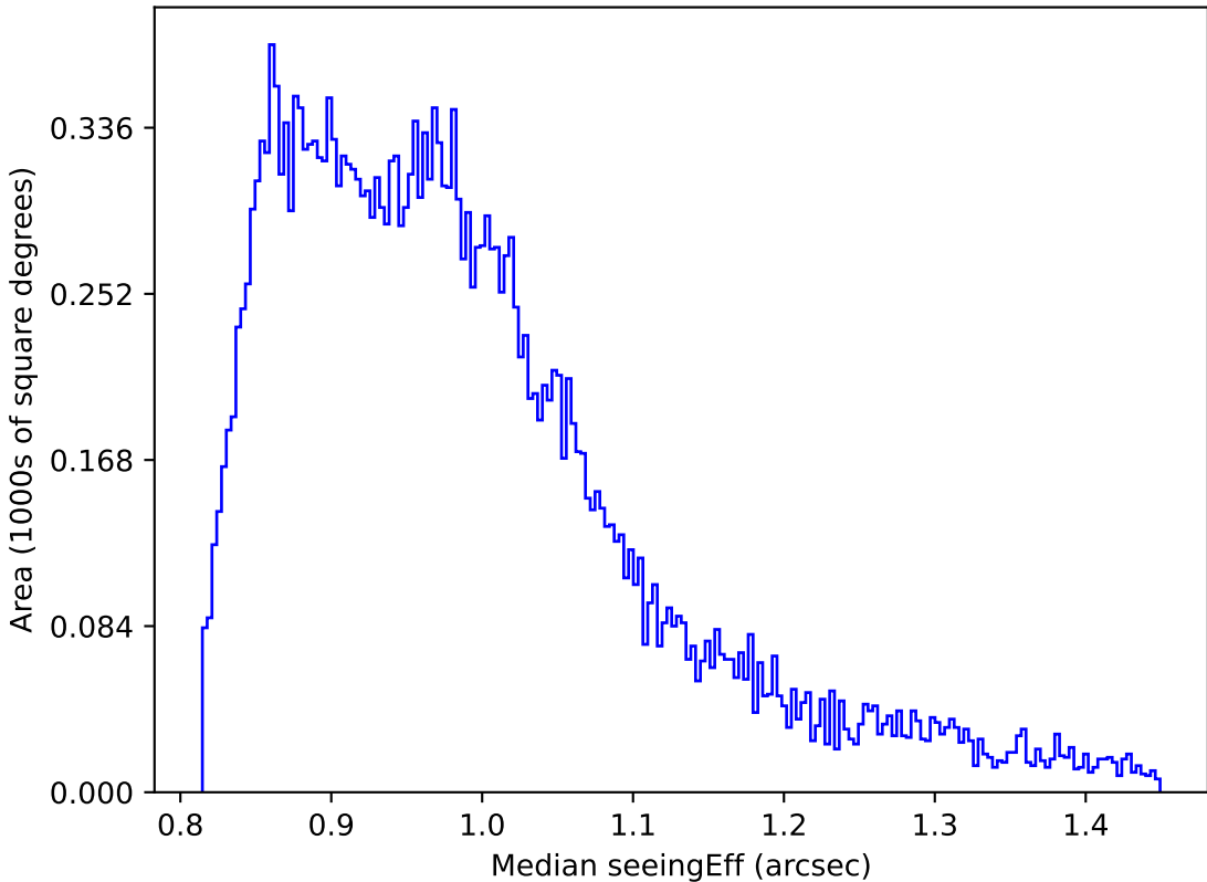
too_elab_r128_d2_gz_v3.4_10yrs Yr 1 all bands: Median seeingEff
