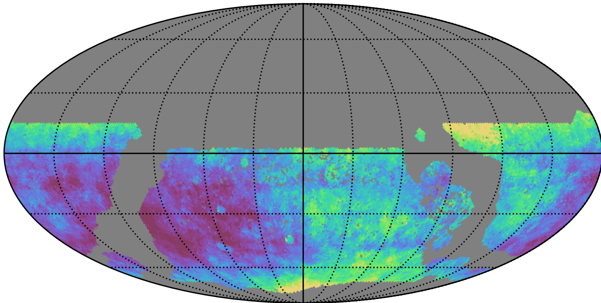
too_elab_r128_d2_gz_v3.4_10yrs WFD z band: Median seeingEff
