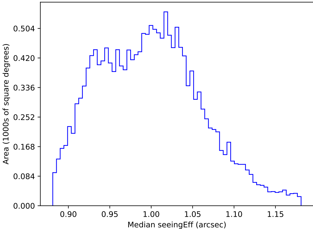
too_elab_r128_d2_gz_v3.4_10yrs WFD y band: Median seeingEff
