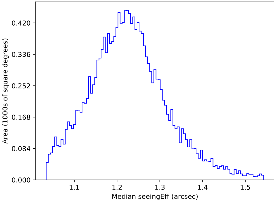
too_elab_r128_d2_gz_v3.4_10yrs WFD u band: Median seeingEff
