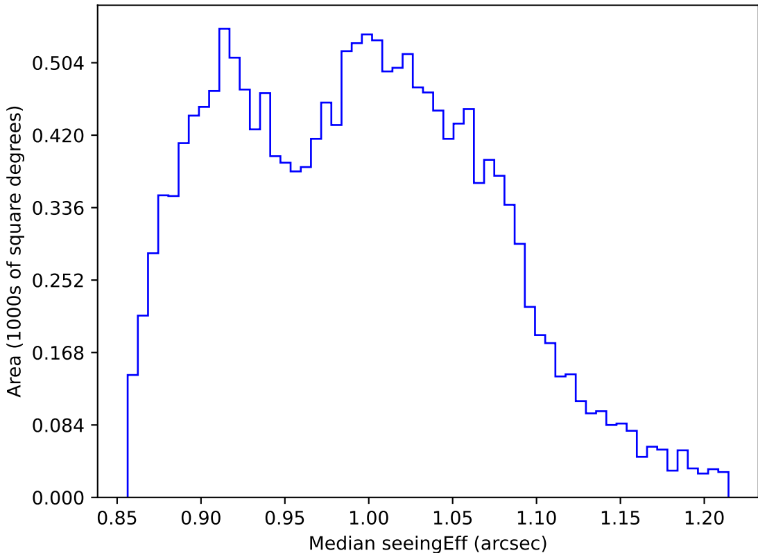
too_elab_r128_d2_gz_v3.4_10yrs WFD i band: Median seeingEff
