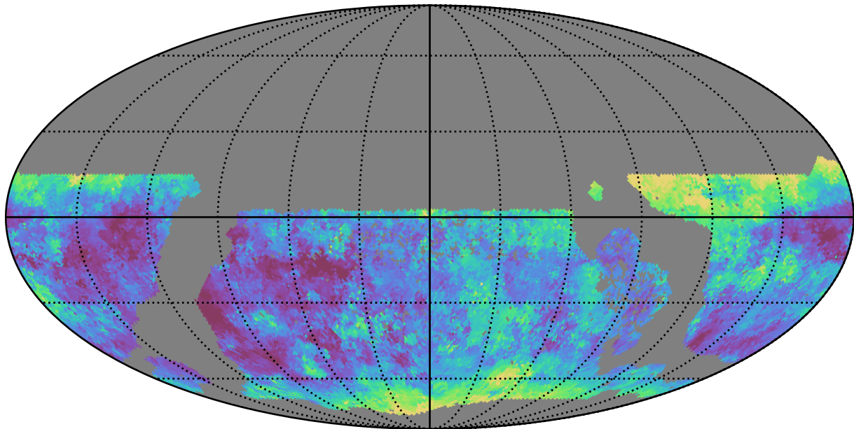
too_elab_r128_d2_gz_v3.4_10yrs WFD g band: Median seeingEff
