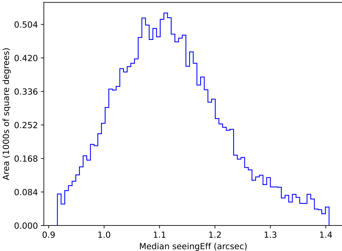
too_elab_r128_d2_gz_v3.4_10yrs WFD g band: Median seeingEff
