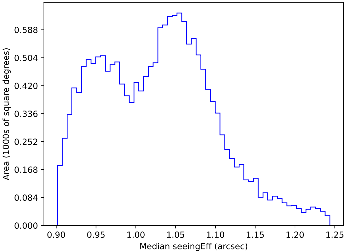
too_elab_r128_d2_gz_v3.4_10yrs WFD all bands: Median seeingEff
