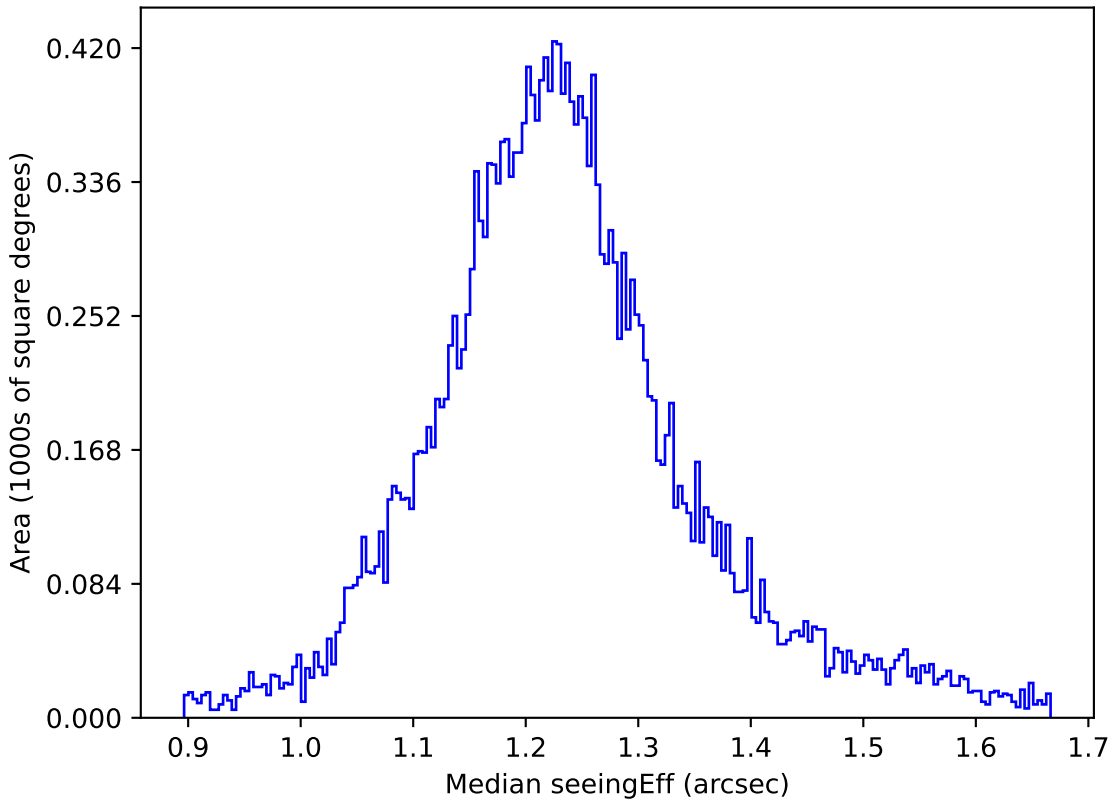
too_elab_r128_d2_gz_v3.4_10yrs All sky u band: Median seeingEff
