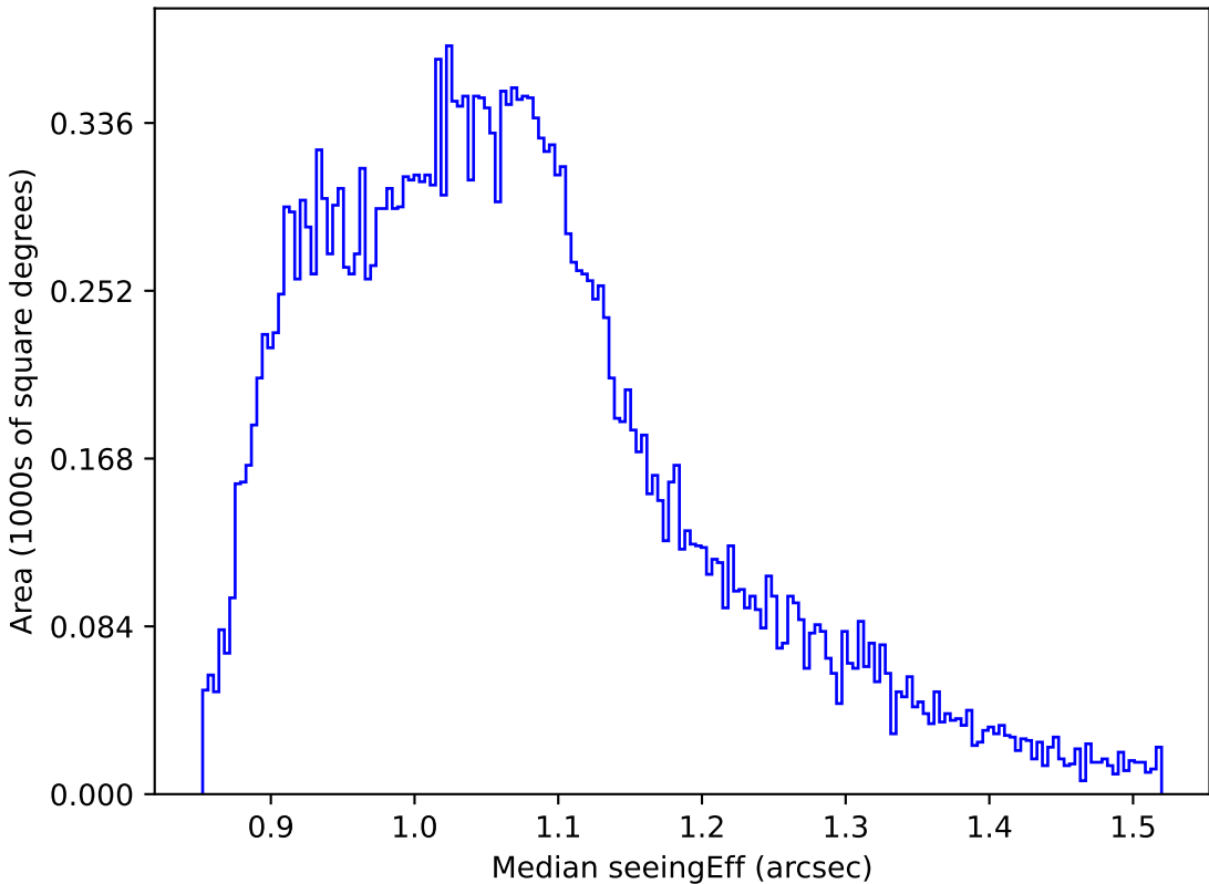
too_elab_r128_d2_gz_v3.4_10yrs All sky r band: Median seeingEff
