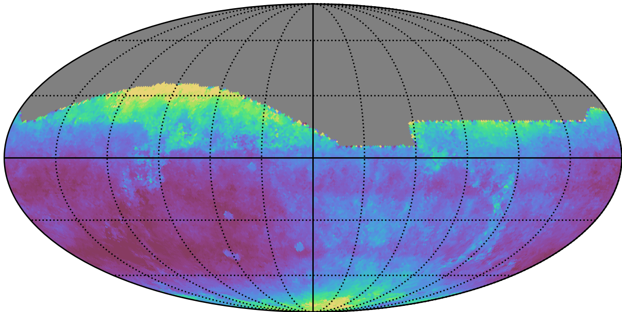
too_elab_r128_d2_gz_v3.4_10yrs All sky i band: Median seeingEff
