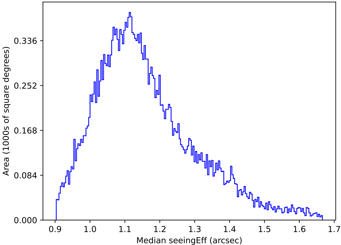
too_elab_r128_d2_gz_v3.4_10yrs All sky g band: Median seeingEff
