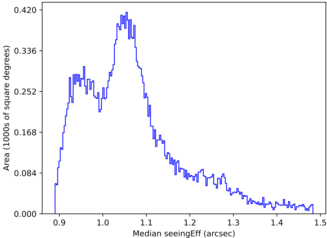
too_elab_r128_d2_gz_v3.4_10yrs All sky all bands: Median seeingEff
