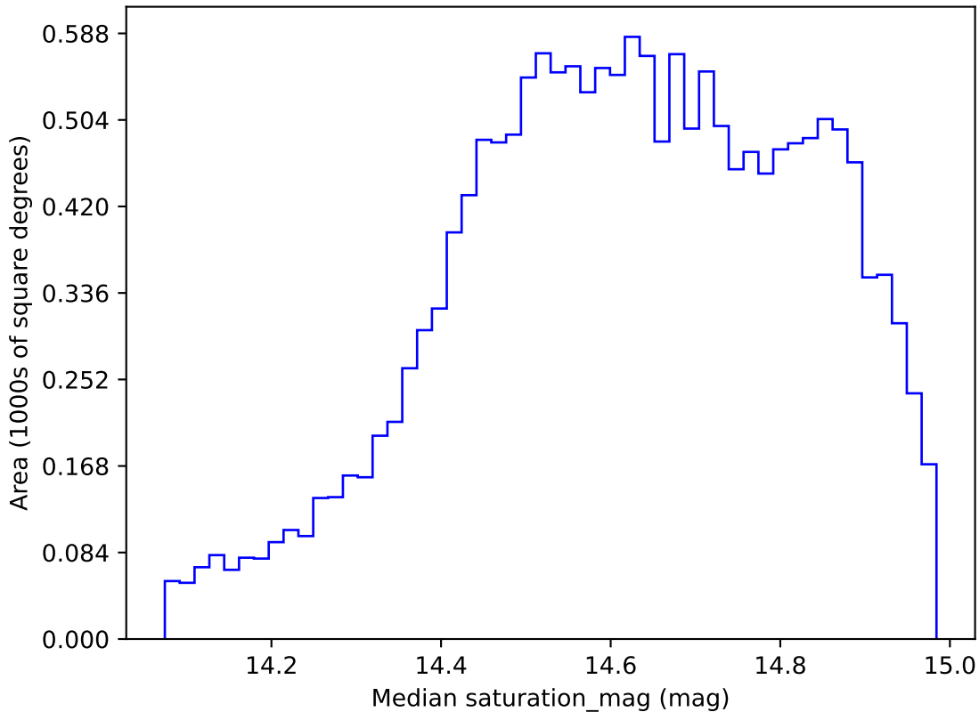
too_elab_r128_d2_gz_v3.4_10yrs WFD r band: Median saturation_mag
