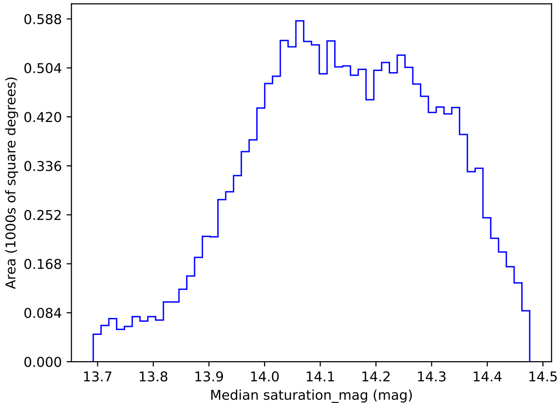
too_elab_r128_d2_gz_v3.4_10yrs WFD all bands: Median saturation_mag
