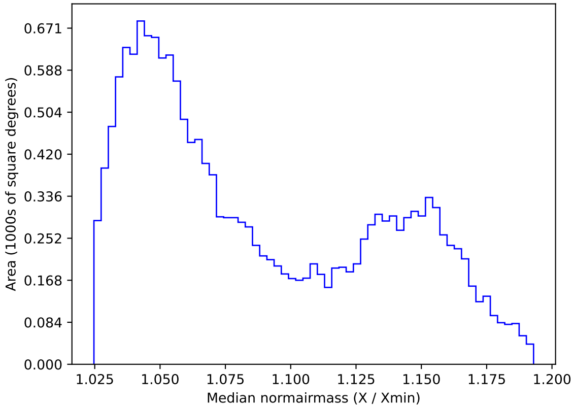
too_elab_r128_d2_gz_v3.4_10yrs WFD z band: Median normairmass
