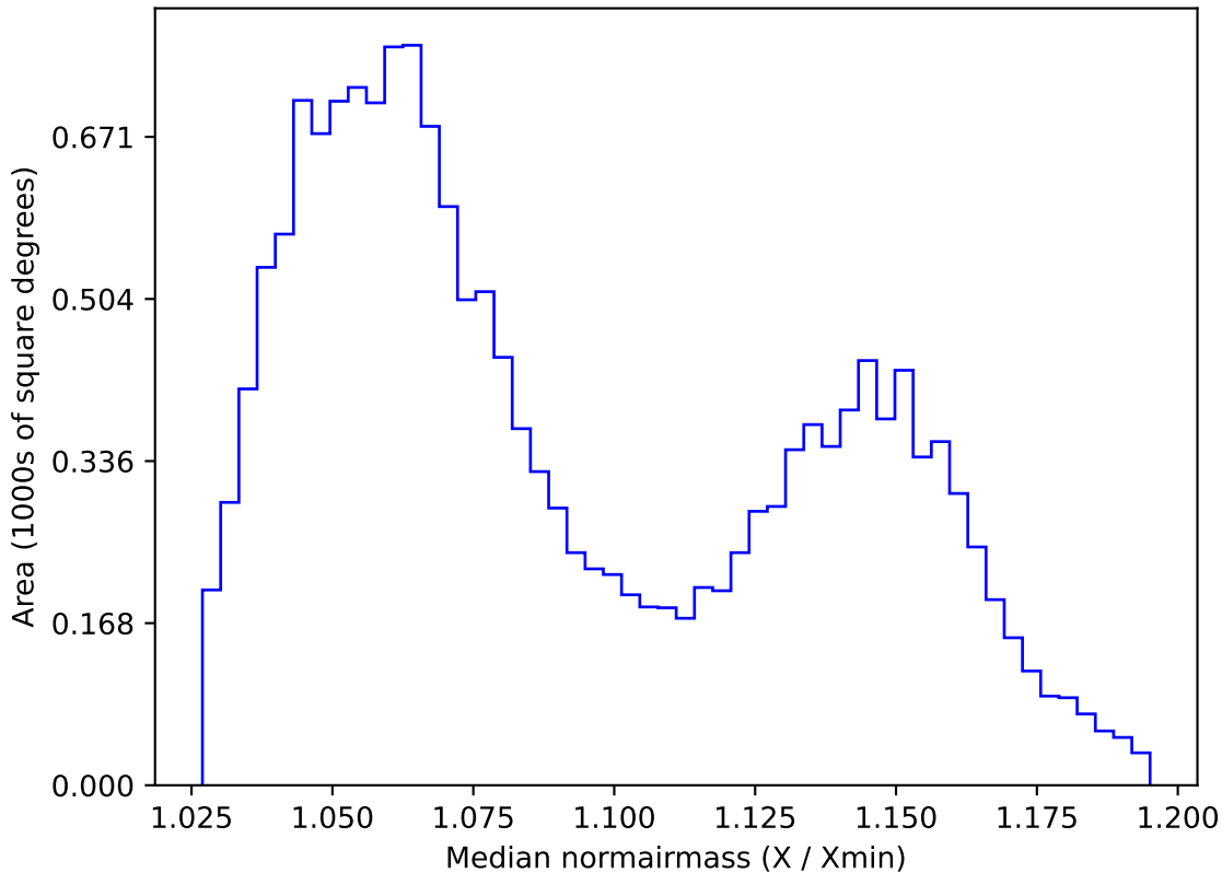
too_elab_r128_d2_gz_v3.4_10yrs WFD y band: Median normairmass
