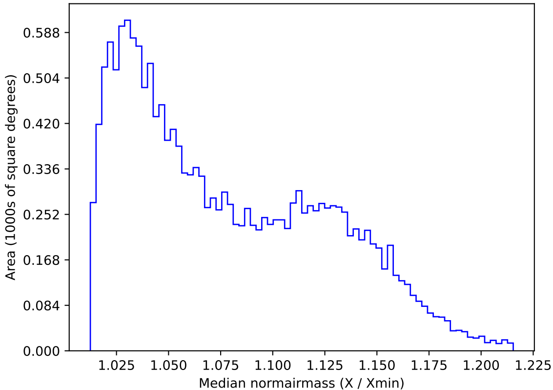
too_elab_r128_d2_gz_v3.4_10yrs WFD u band: Median normairmass
