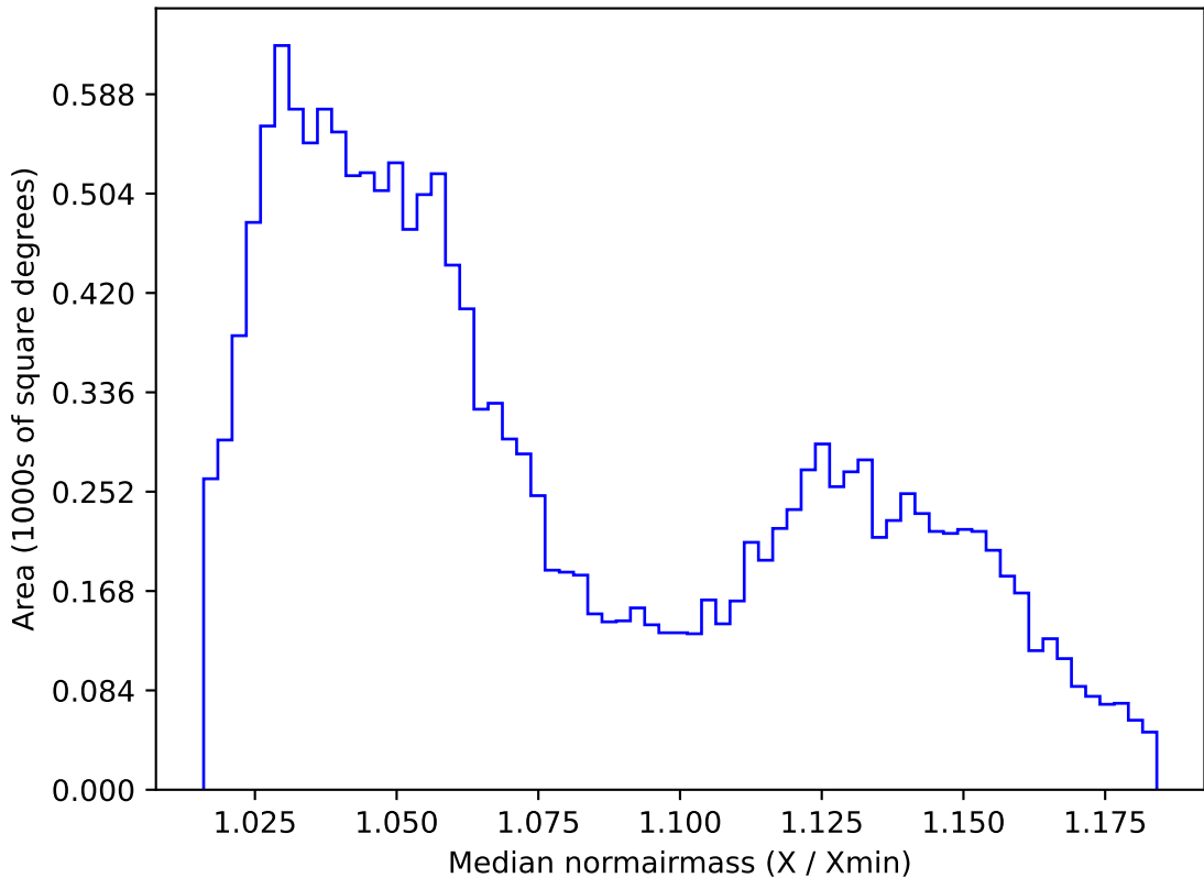
too_elab_r128_d2_gz_v3.4_10yrs WFD r band: Median normairmass
