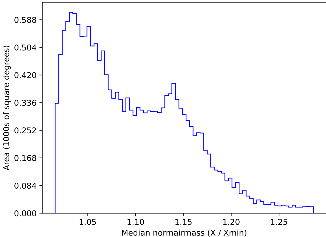
too_elab_r128_d2_gz_v3.4_10yrs WFD g band: Median normairmass
