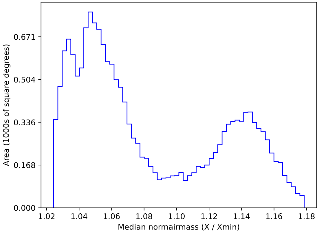
too_elab_r128_d2_gz_v3.4_10yrs WFD all bands: Median normairmass
