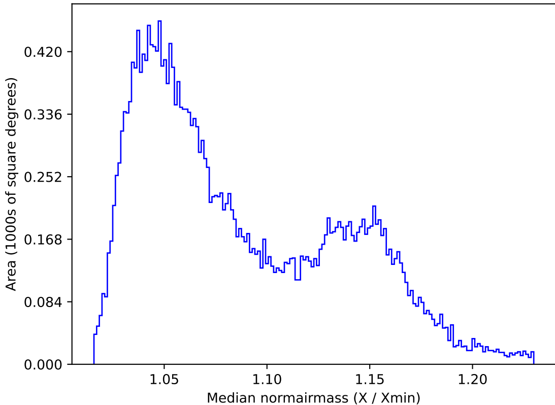
too_elab_r128_d2_gz_v3.4_10yrs All sky z band: Median normairmass
