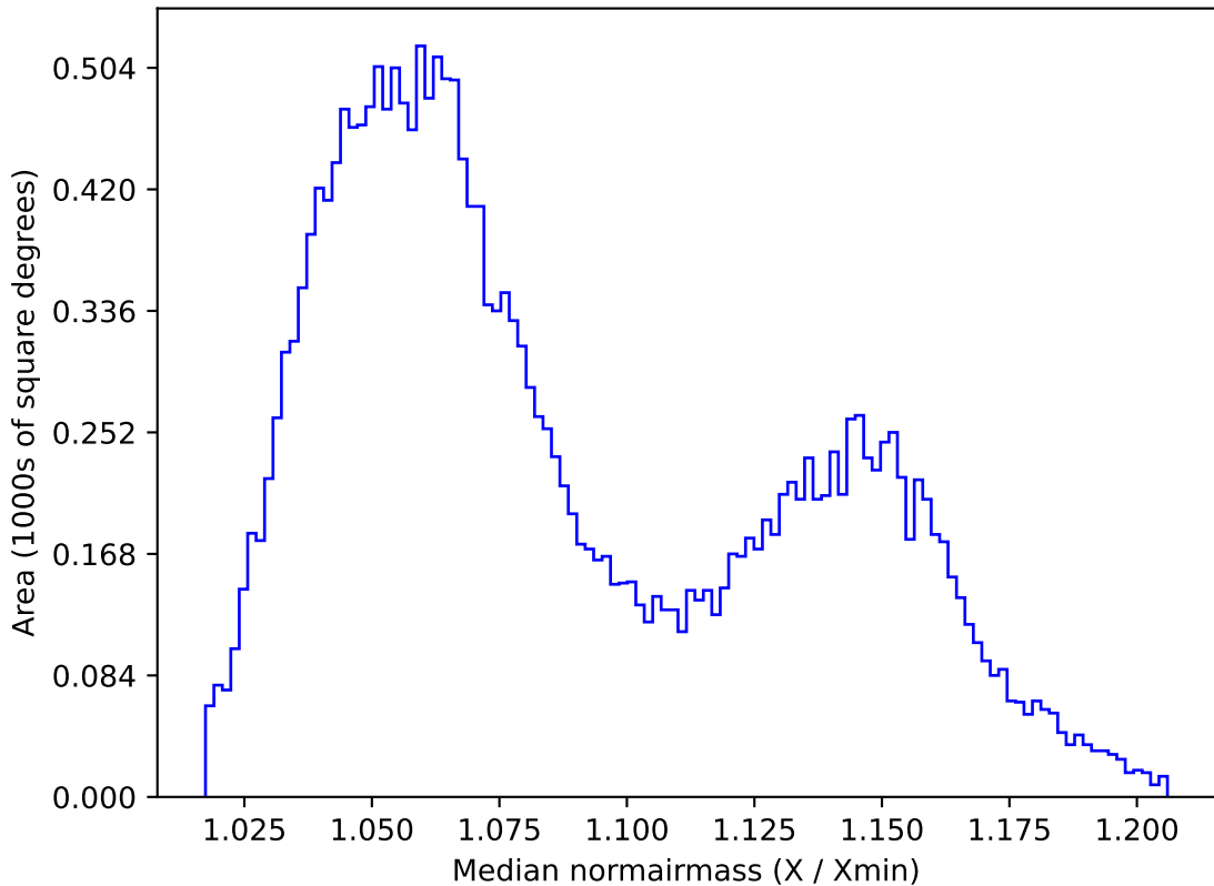
too_elab_r128_d2_gz_v3.4_10yrs All sky y band: Median normairmass
