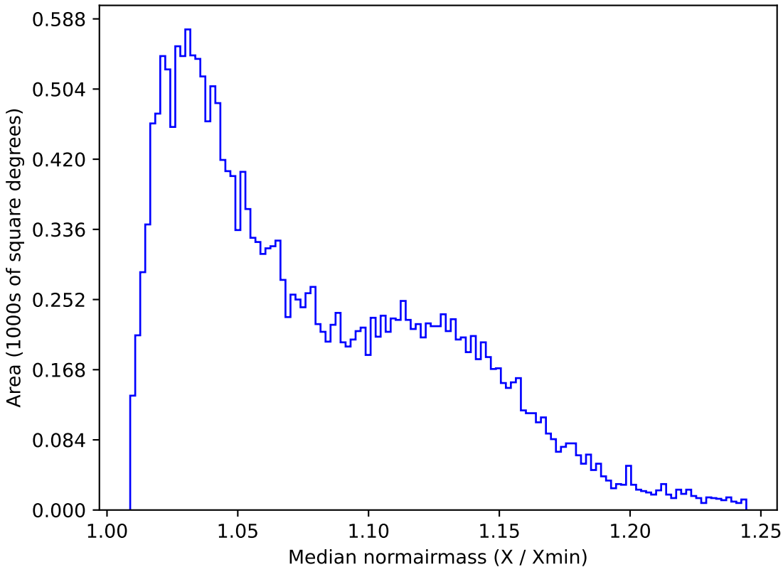
too_elab_r128_d2_gz_v3.4_10yrs All sky u band: Median normairmass
