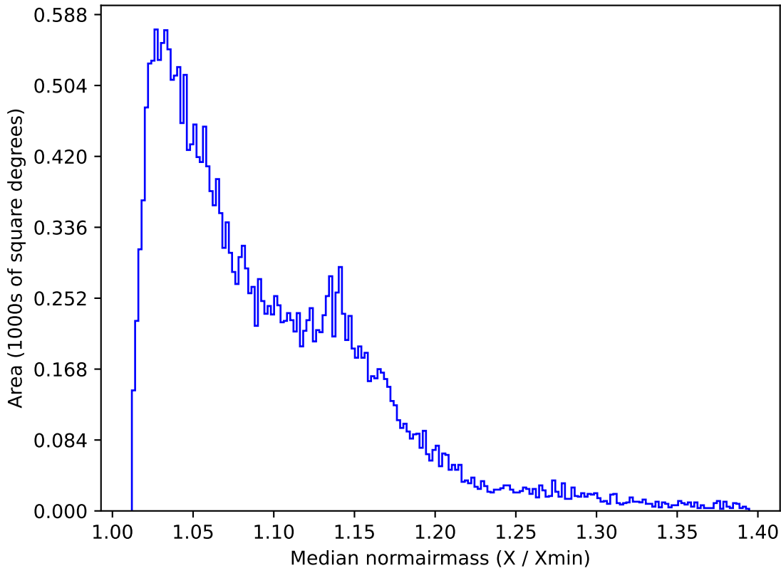
too_elab_r128_d2_gz_v3.4_10yrs All sky g band: Median normairmass
