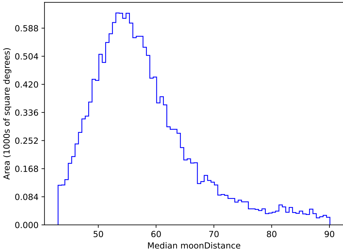
too_elab_r128_d2_gz_v3.4_10yrs WFD y band: Median moonDistance
