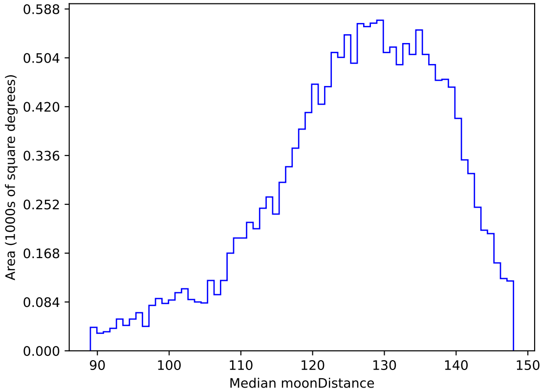
too_elab_r128_d2_gz_v3.4_10yrs WFD u band: Median moonDistance
