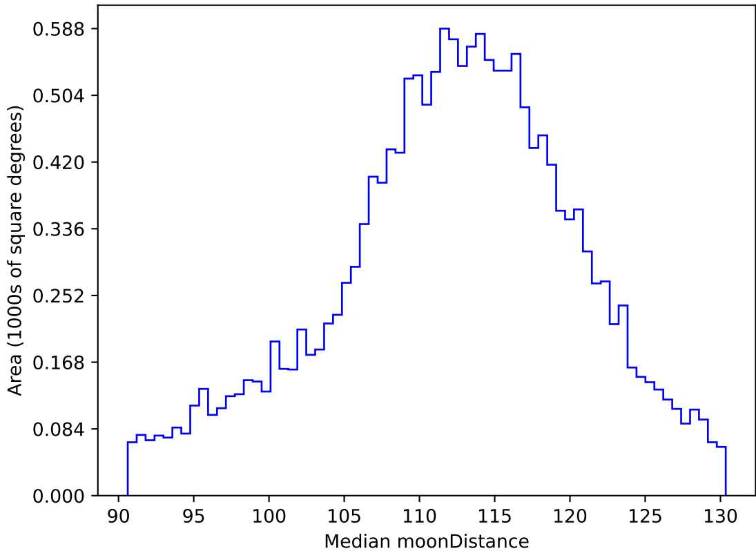
too_elab_r128_d2_gz_v3.4_10yrs WFD r band: Median moonDistance
