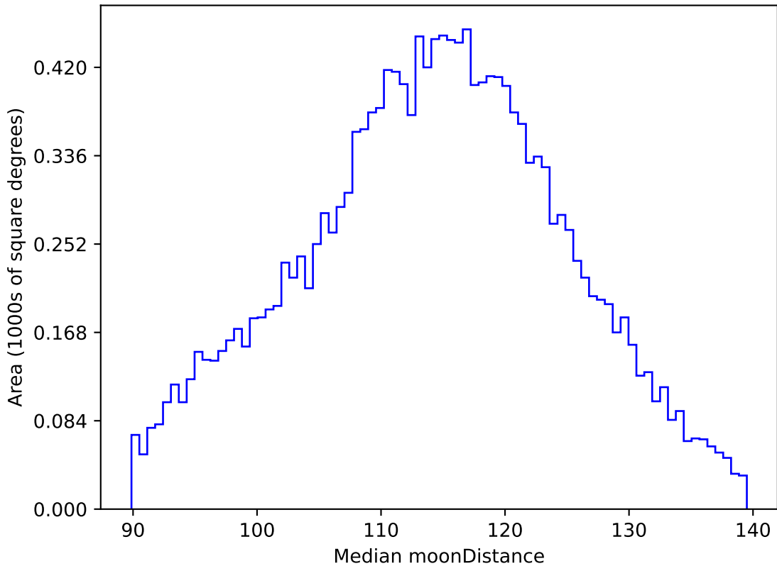
too_elab_r128_d2_gz_v3.4_10yrs WFD g band: Median moonDistance
