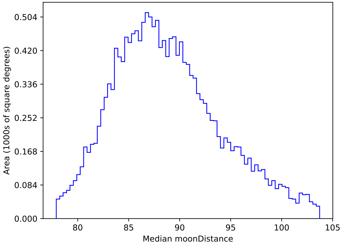
too_elab_r128_d2_gz_v3.4_10yrs WFD all bands: Median moonDistance
