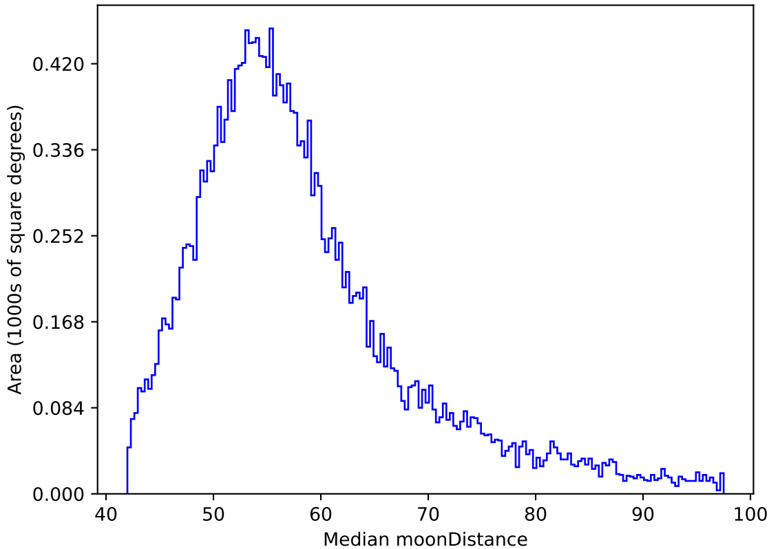
too_elab_r128_d2_gz_v3.4_10yrs All sky y band: Median moonDistance
