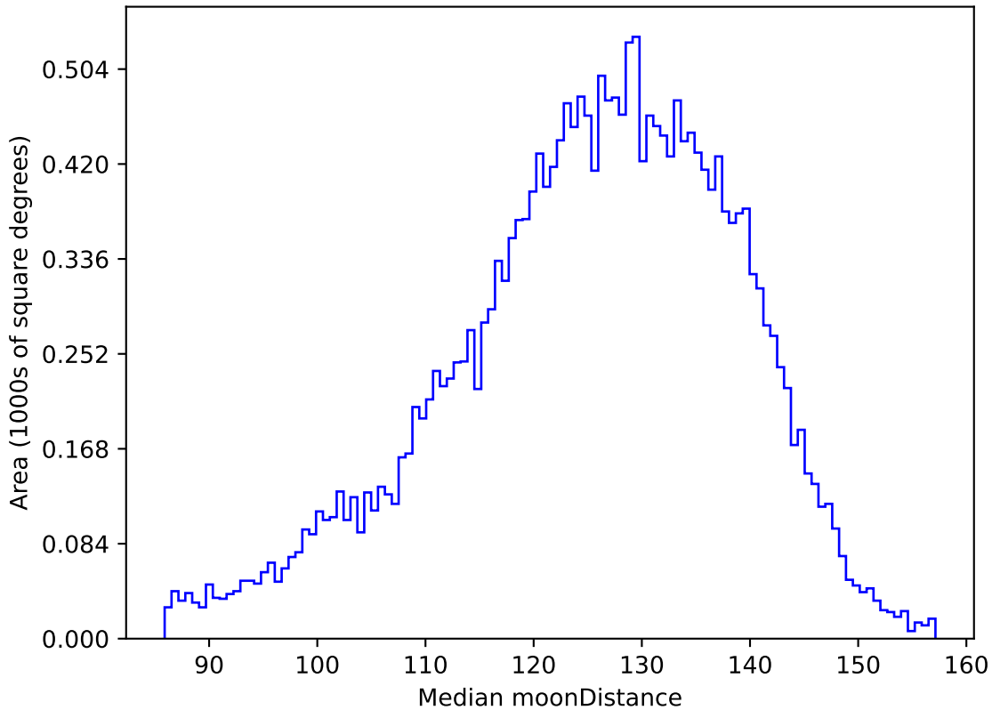
too_elab_r128_d2_gz_v3.4_10yrs All sky u band: Median moonDistance
