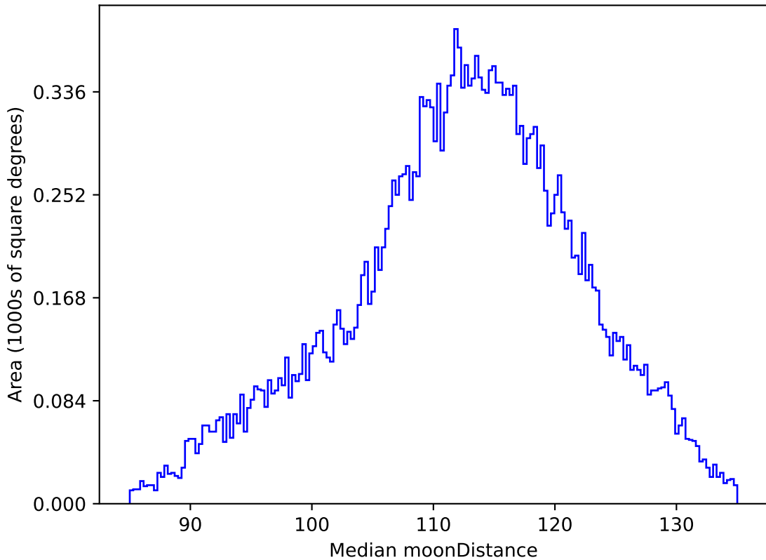
too_elab_r128_d2_gz_v3.4_10yrs All sky r band: Median moonDistance
